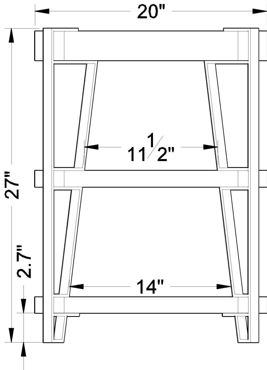
FRONT VIEW
