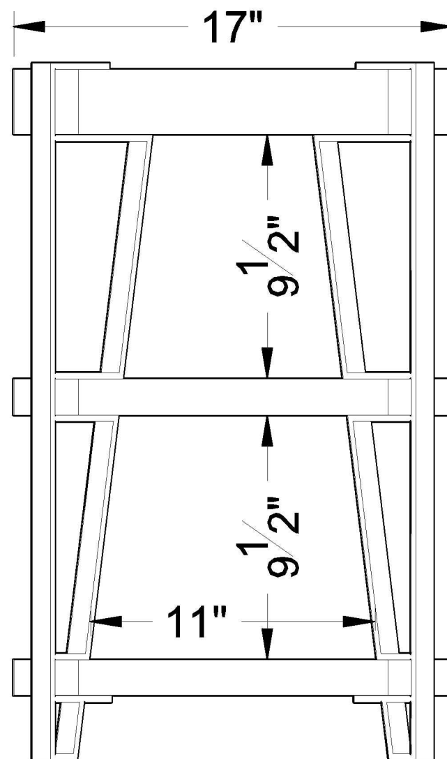
SIDE VIEW
