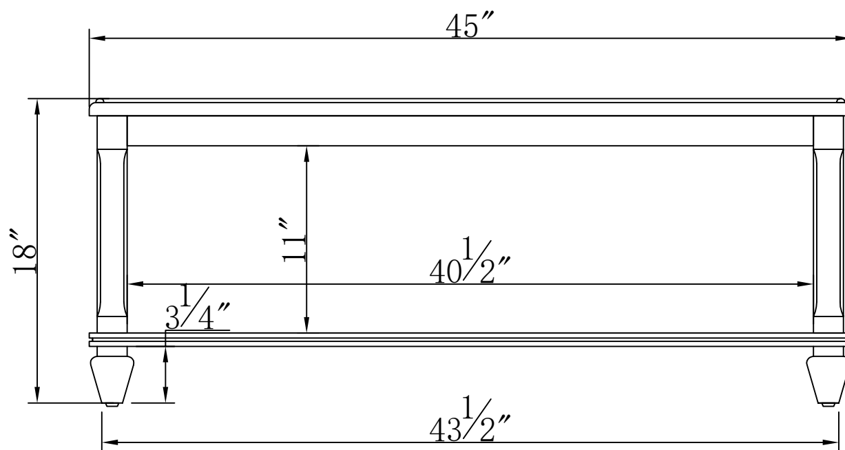
ANSB1162 26"X45" COFFEE TABLE
