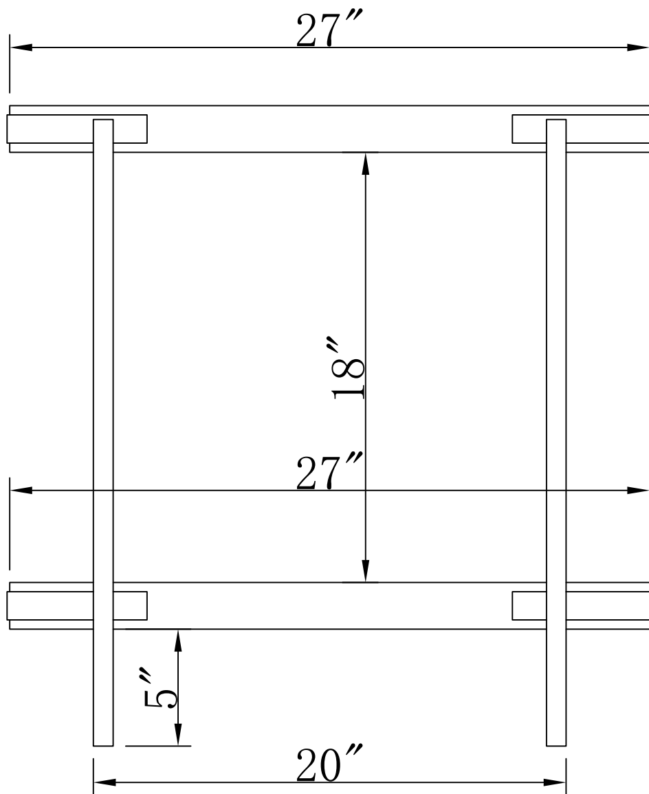
FRONT VIEW
